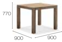
Teak Square Table _ 659571
